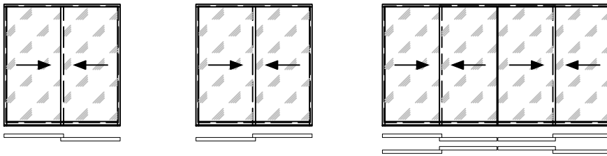
3-bahnig / 3-rails
